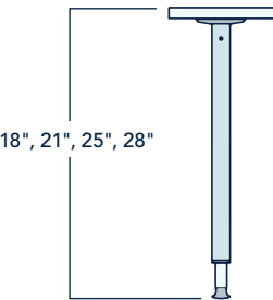
Fixed Height Overall Table Heights Standard Height: 28 inch Optional Low Heights: 18 inch, 21 inch & 25 inch
