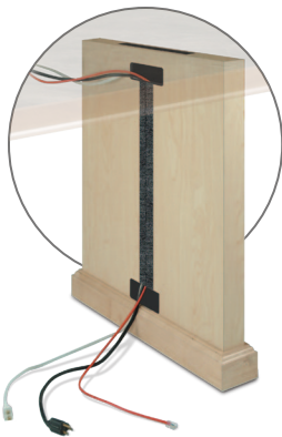
Optional Race Panel Wire Management
