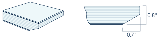
Edge Model BP1: Knife Profile Baltic Birch Plywood
