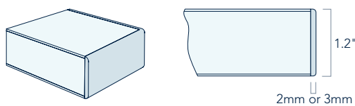
Edge Model PK4: Knife Profile Edgeband
