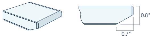
Edge Model PK1: Knife Profile Edgeband
