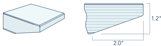
Edge Model BP4: Knife Profile Baltic Birch Plywood
