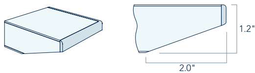
Edge Model PK4: Knife Profile Edgeband
