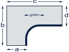
Extended Corner Right
