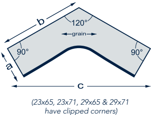
120° Corner W/ 90° Ends
