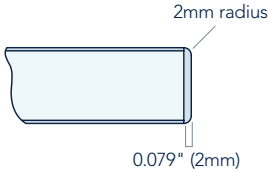
2mm Edgeband Flat Profile
