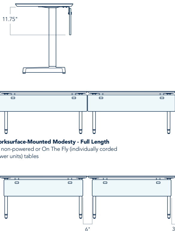
Worksurface-Mounted Modesty 6" undersize for Move About (consecutively powered) tables
